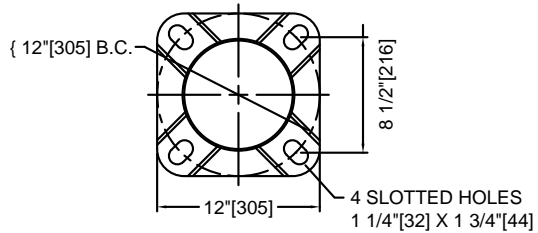
ANCHOR BASE
