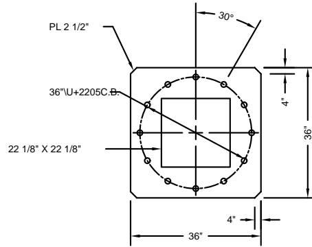
ANCHOR BASE (FOR 1 1/2"Ø X 81"LG A.B.)
