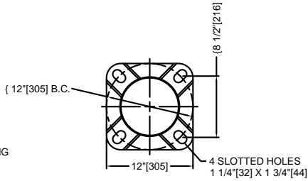
ANCHOR BASE
